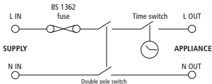
Fig. 3 Internal Schematic of FST17A/FST11A
